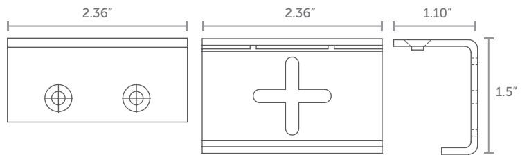
Heavy Duty 105 Bracket RX-268
